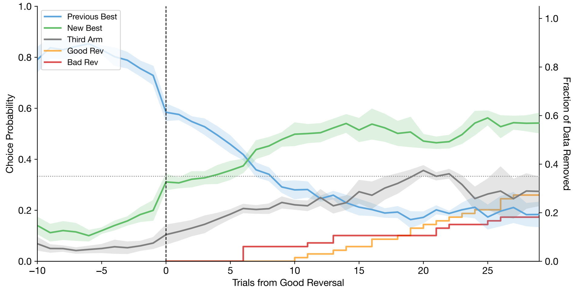
Good Reversal-Aligned Choices (mean \pm se across subjects | n=6 subjects, n=66 reversals)
